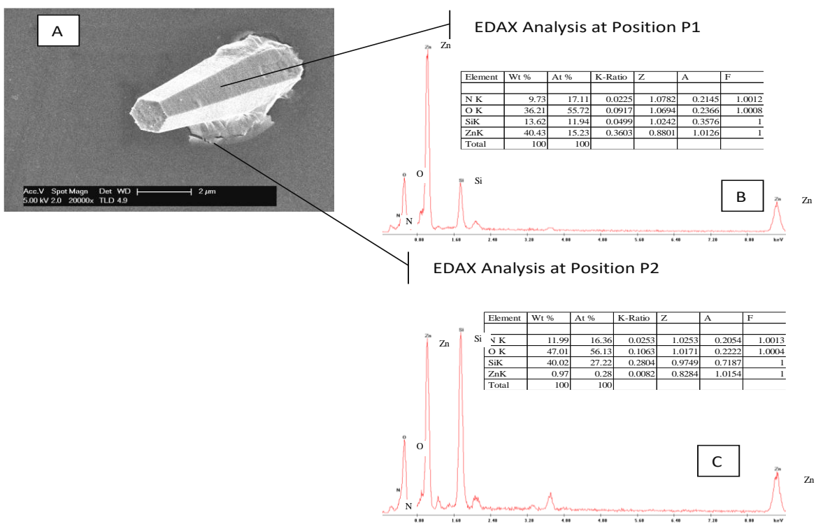
Fig.7: A: SEM image (top view) of N1:S1-MS; B: EDX analysis at position P1 (X-shaped ZnO crystal); C: EDX analysis at position P2 (layer upon magnetron sputtered coating and small ZnO crystal) at high concentration of TEA with pH control.
