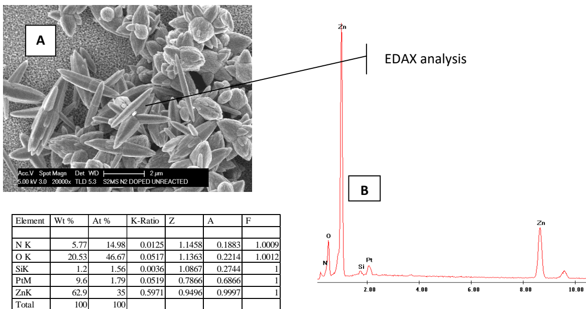
Fig. 5: A: SEM image (top view) of N:S2-MS; B: EDX analysis at position P1(complex ZnO single crystal).
