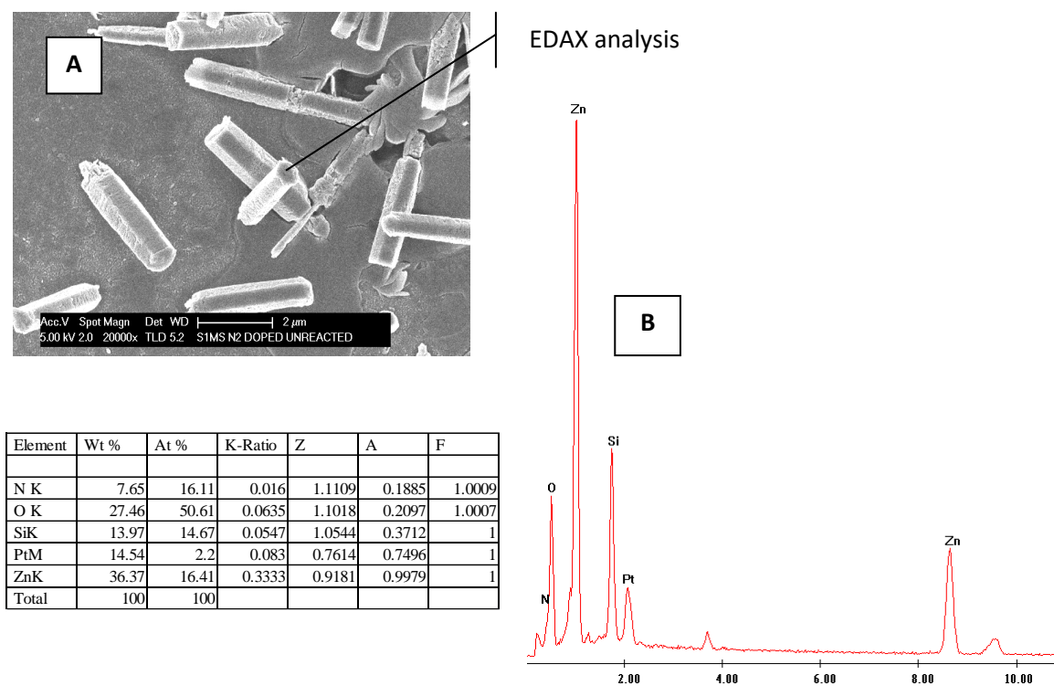
Fig. 3: (A): SEM image (top view) of nitrogen-doped nanostructured ZnO thin films N1:S1-MS; (B) :EDX analysis at position P1(ZnO single crystal).
