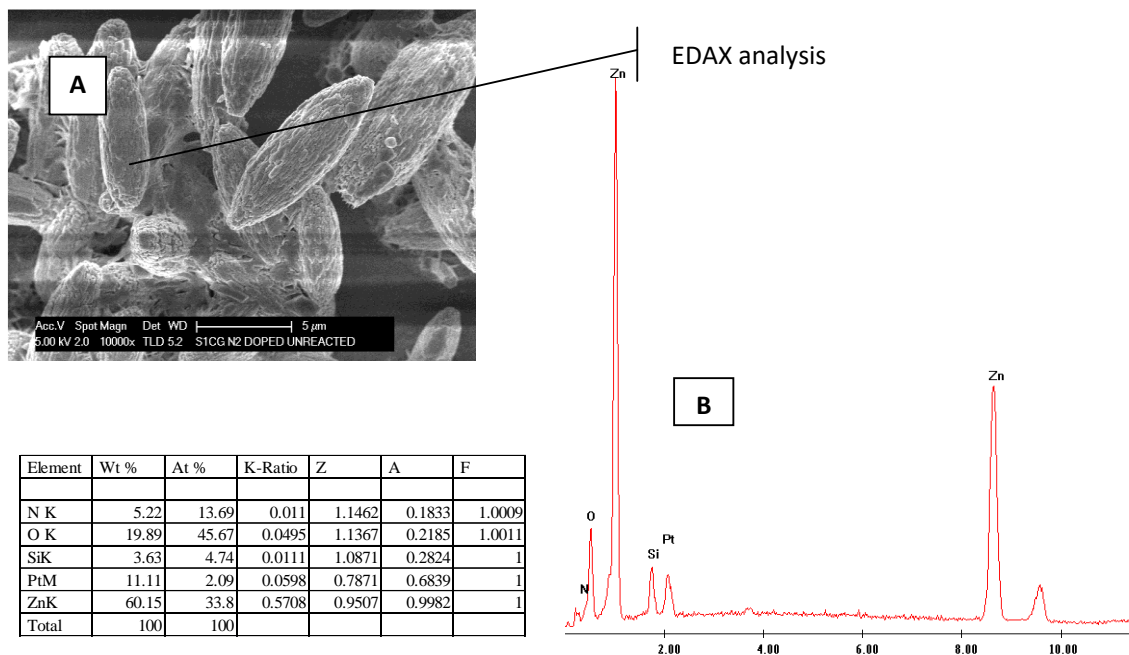
Fig. 4: A: SEM image (top view) of N:S1-CG; B:EDX analysis at position P1(ZnO single crystal).
