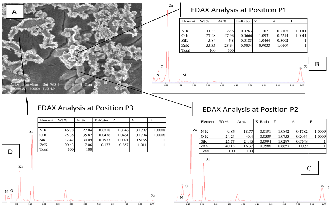
Fig. 9: A: SEM image (top view) of N2:S2-MS; B: EDX analysis at position P1(cluster of ZnO crystal); C: EDX analysis at position P2(ZnO single crystal); D: EDX analysis of at position P3 (layer upon magnetron sputtered coating).
