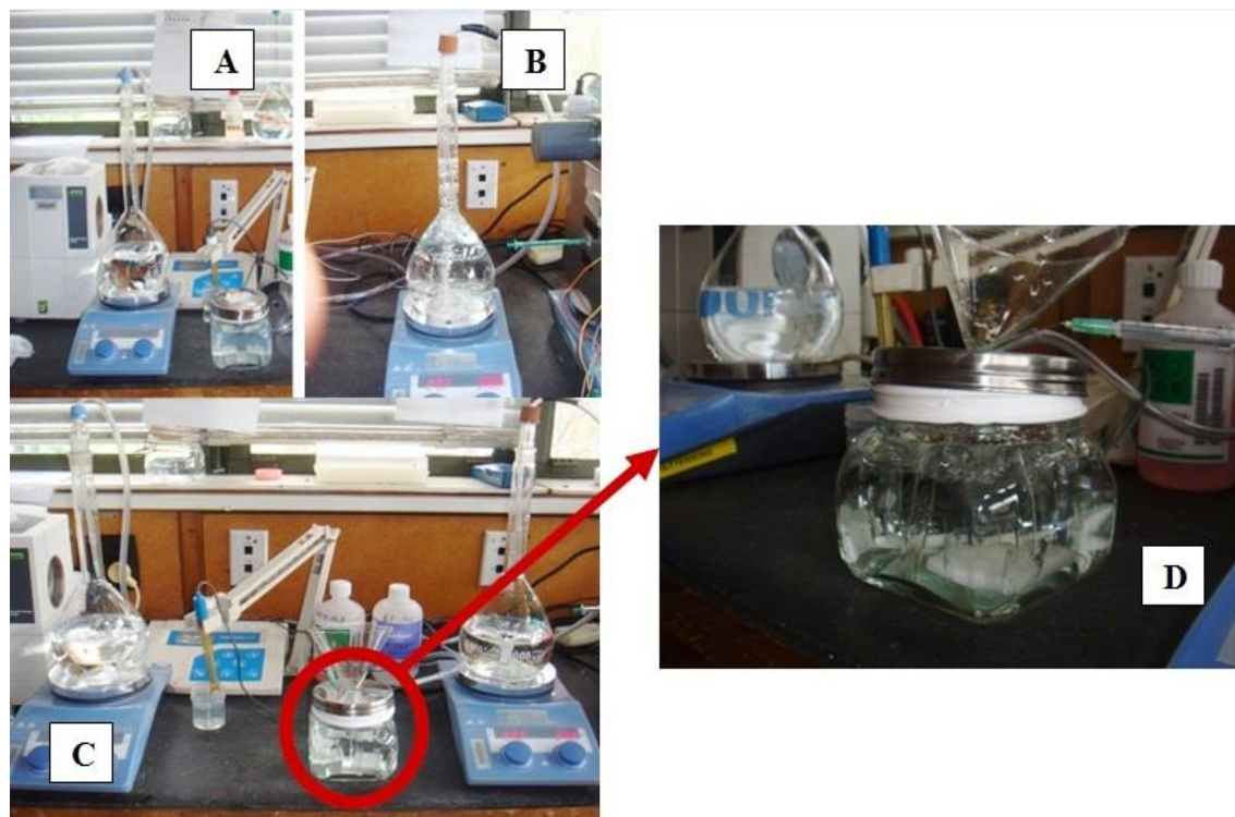
Fig. 1: Preparation of N:ZnO by using N 2 gas as nitrogen dopant source: (A) N 2 saturated Zn(NO 3 ) 2 ·6H 2 O; (B) N 2 saturated HMT; (C) Mixing of N 2 saturated Zn(NO 3 ) 2 ·6H 2 O and HMT under extensive supply of N 2 ; (D) Magnified view of sealable glass jar
