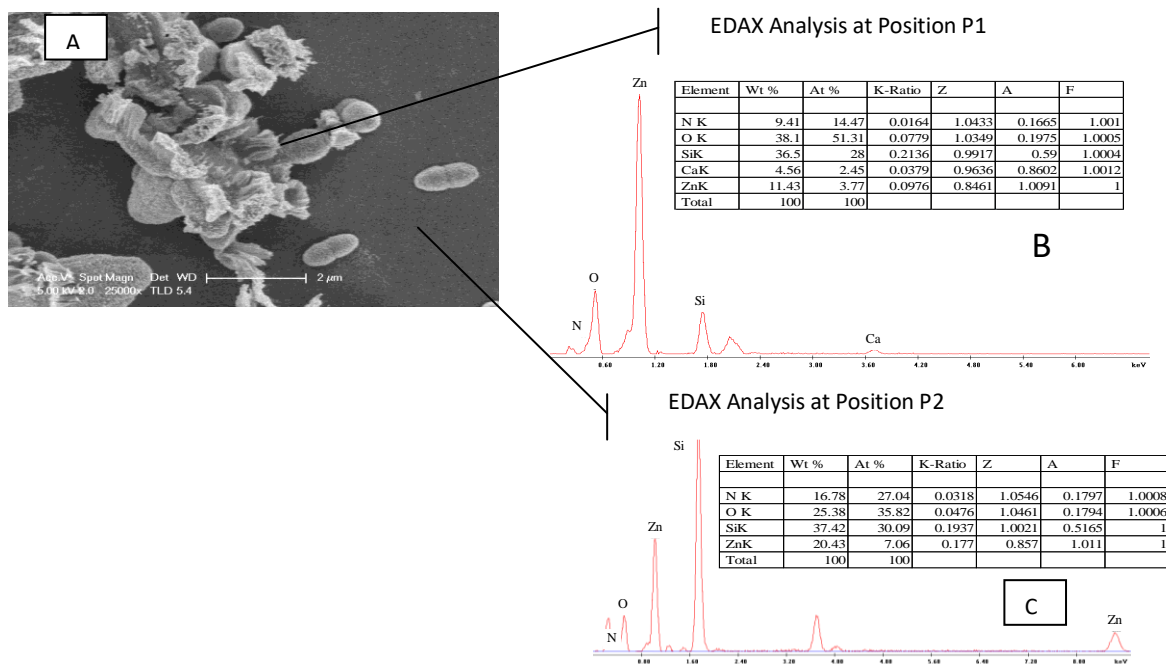
Fig. 12: A: SEM image (top view) of N4:S2-MS; B: EDX analysis at position P1(cluster of ZnO crystal); C: EDX analysis at position P2(layer upon magnetron sputtered coating).
