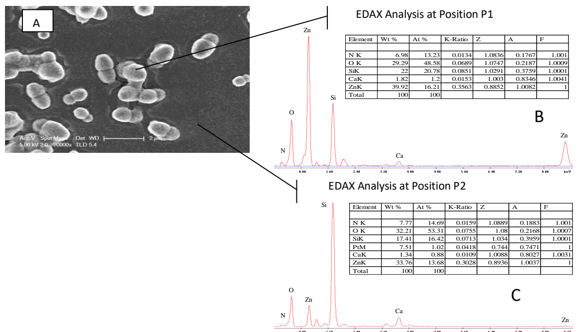
Fig. 13: A: SEM image (top view) of N4:S2-CG; B: EDX analysis at position P1(ZnO jointed crystal); C: EDX analysis at position P2 (layer upon magnetron sputtered coating) at low concentration of TEA with pH control.
