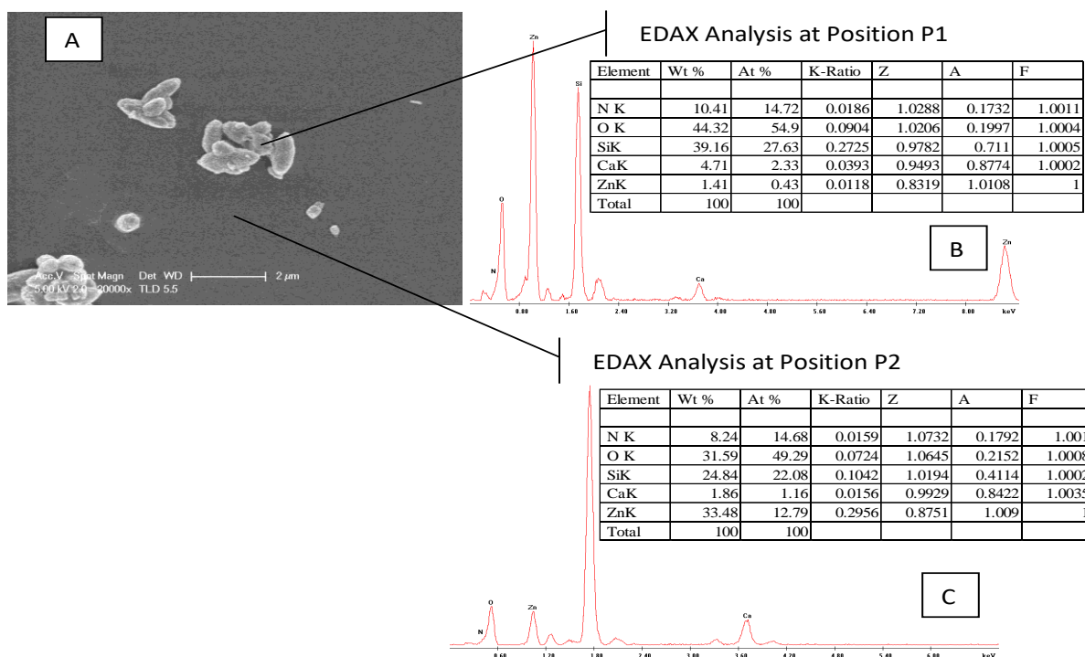
Fig. 14: A: SEM image (top view) of N5:S2-MS; B: EDX analysis at position P1(cluster of ZnO crystal); C:EDX analysis at position P2(layer upon magnetron sputtered coating) at high concentration of TEA without pH control.
