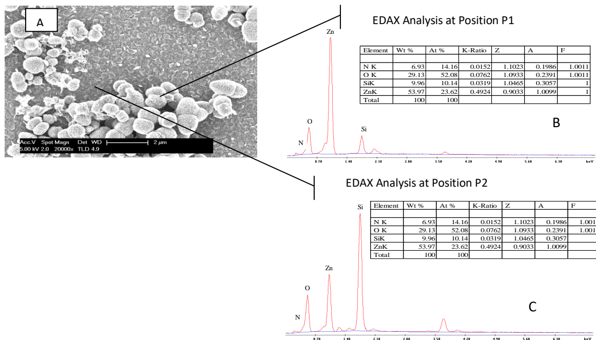
Fig. 16: A: SEM image (top view) of N6:S2-MS; B:EDX analysis at position P1(cluster of ZnO crystal); C:EDX analysis at position P2(flowery layer upon magnetron sputtered coating) at low concentration of TEA without pH control.
