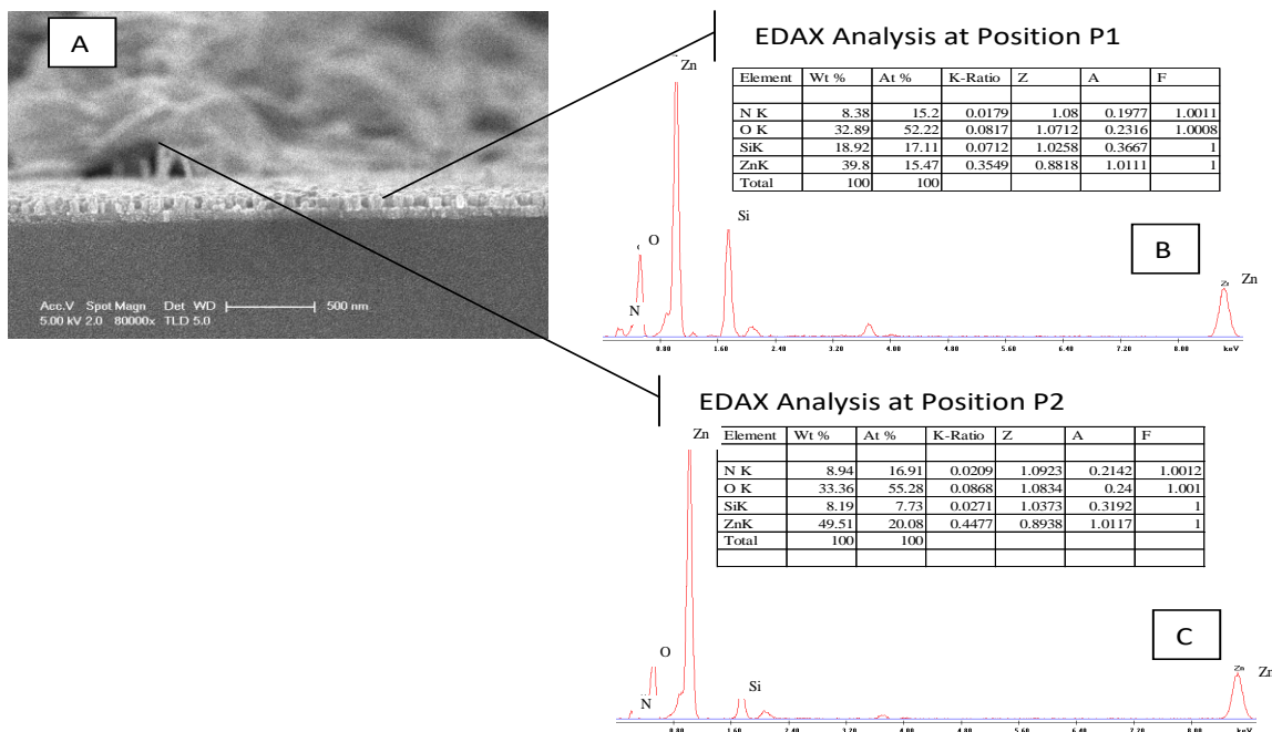
Fig. 10: A: SEM image (cross-sectional) of N2:S2-MS; B: EDX analysis at position P1 (cluster of ZnO crystal); C: EDX analysis at position P2(complex ZnO single crystal).
