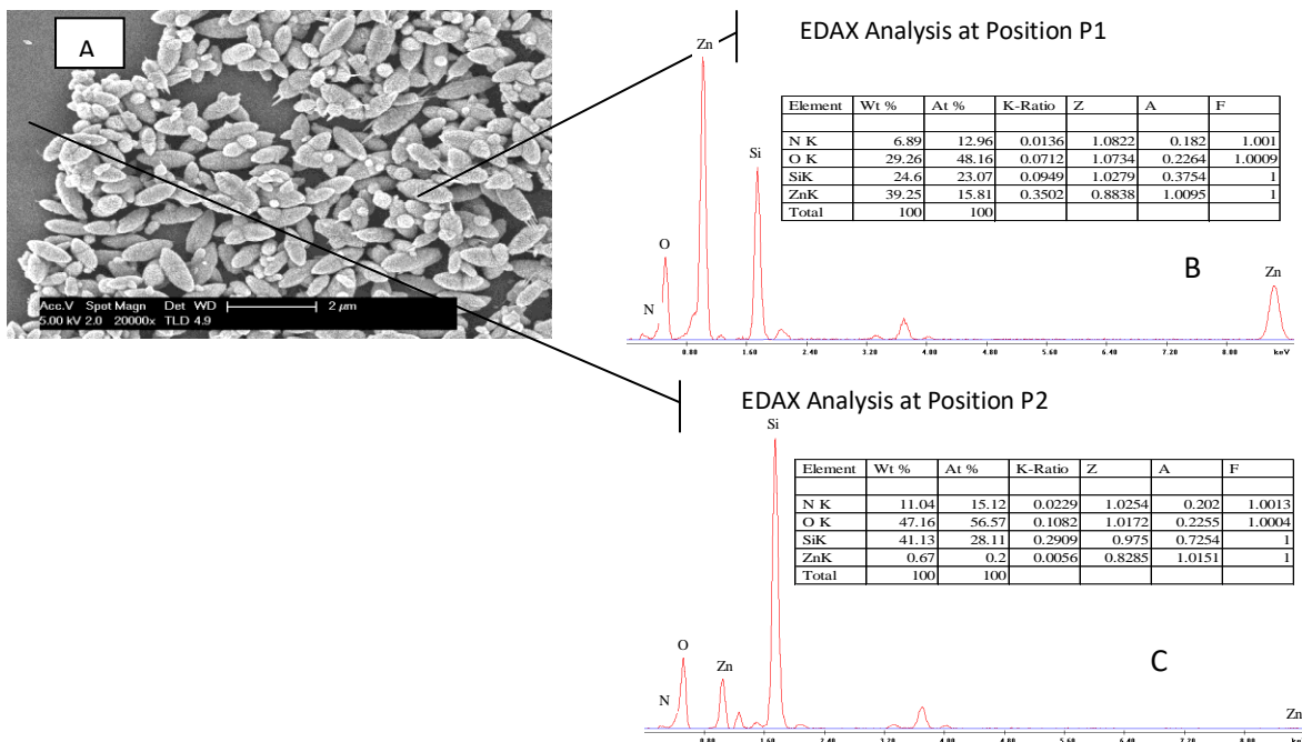
Fig. 15: A: SEM image (top view) of N5:S2-CG; B:EDX analysis at position P1(edged ZnO crystal); C:EDX analysis at position P2(layer upon magnetron sputtered coating) at high concentration of TEA without pH control.
