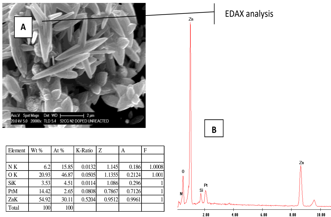
Fig.6: A: SEM image (top view) of N:S2-CG; B: EDX analysis at position P1 (complex ZnO single crystal).
